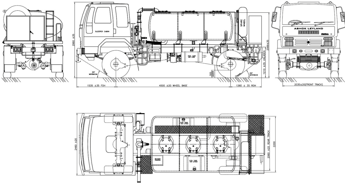
STALLION WATER BOWSER VEHICLE GENERAL ARRANGEMENT
